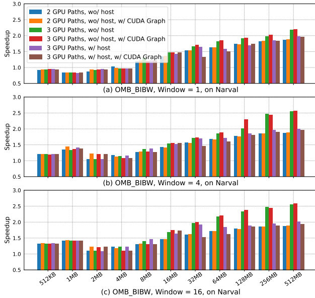
Figure 10: Multi-Path OMB Bidirectional MPI Bandwidth (BIBW) comparison with and without CUDA Graph, on Narval
