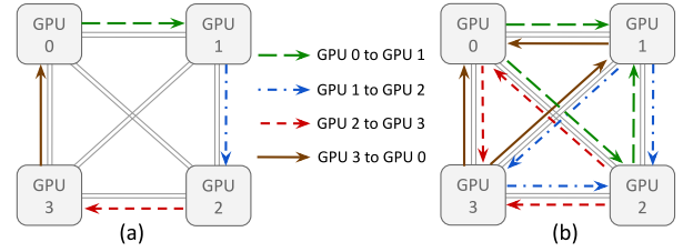
Figure 11: Jacobi communication pattern (a) without multi-path, and (b) with multi-path (two paths per communication) on a four-GPU node
