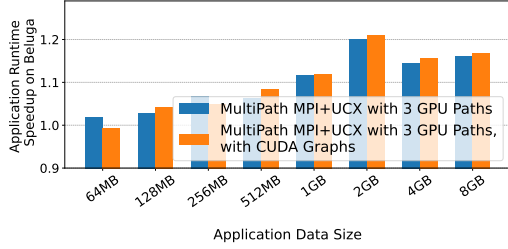
(b) Beluga with three GPU paths
