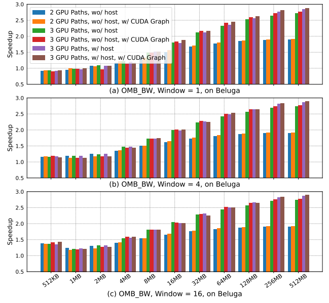
Figure 7: Multi-Path OMB Unidirectional MPI Bandwidth (BW) comparison with and without CUDA Graph, on Beluga
