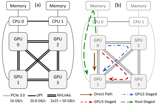
Figure 2: (a) A typical four-GPU node with NVLink (two sub-links) per GPU pair, (b) A communication between GPU-0 and GPU-1 is split and transferred through multiple paths
