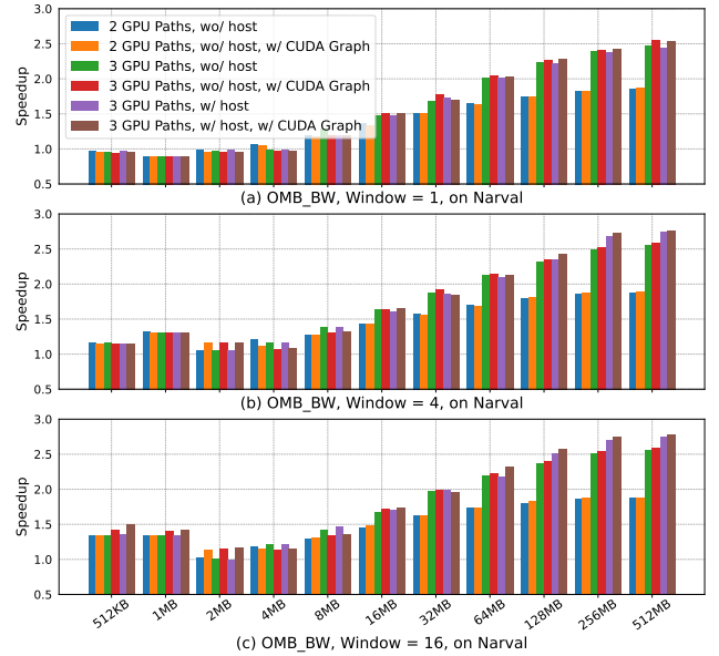
Figure 8: Multi-Path OMB Unidirectional MPI Bandwidth (BW) comparison with and without CUDA Graph, on Narval
