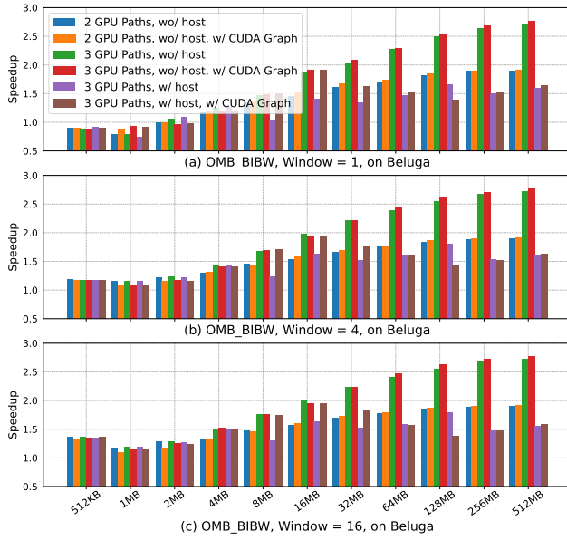
Figure 9: Multi-Path OMB Bidirectional MPI Bandwidth (BIBW) comparison with and without CUDA Graph, on Beluga
