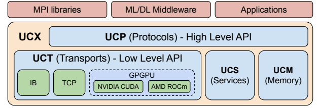
Figure 1: UCX architecture and some of its components
