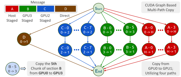
Figure 5: A CUDA Graph-based multi-path communication from GPU-0 to GPU-1 using the available NVLinks and PCIe. The graph in this figure is generated by the CUDA Graph Engine shown in Figure 3. Each node denotes a memory-copy operation, and edges represent the control-flow dependencies ensuring staged transfers execute in the required order.
