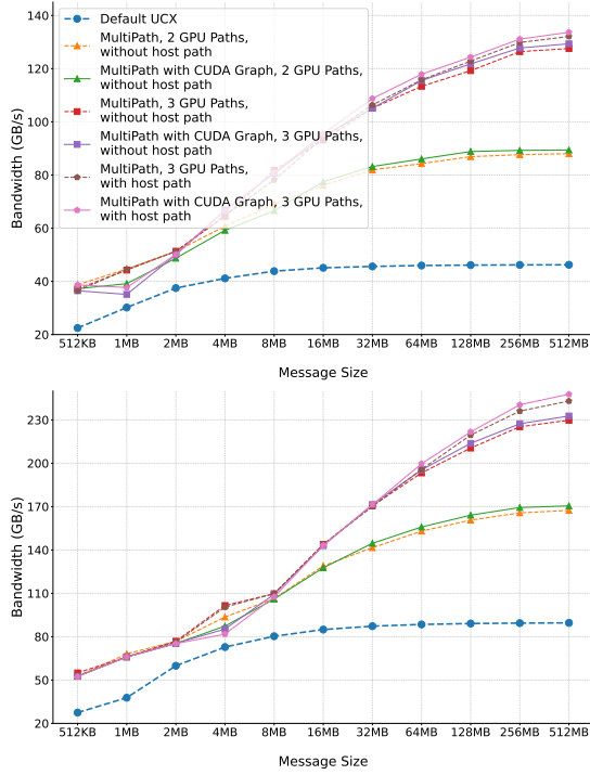
Figure 6: UCX Put Bandwidth comparison of our multi-path framework with and without CUDA Graph against default UCX (UCT::CUDA-IPC), on Beluga (top) and Narval (bottom)
